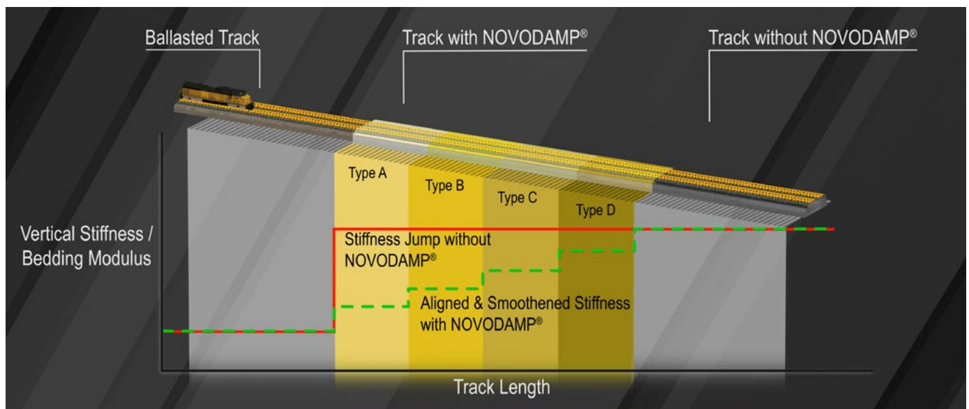
SRT DOUBLE TRACK | BALLASTED TRACK AT TRANSITION ZONES (BRIDGE / APPROACH SLAB), THAILAND
